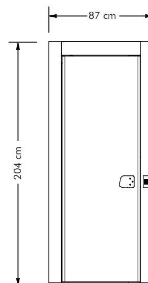
Vista Frontal
